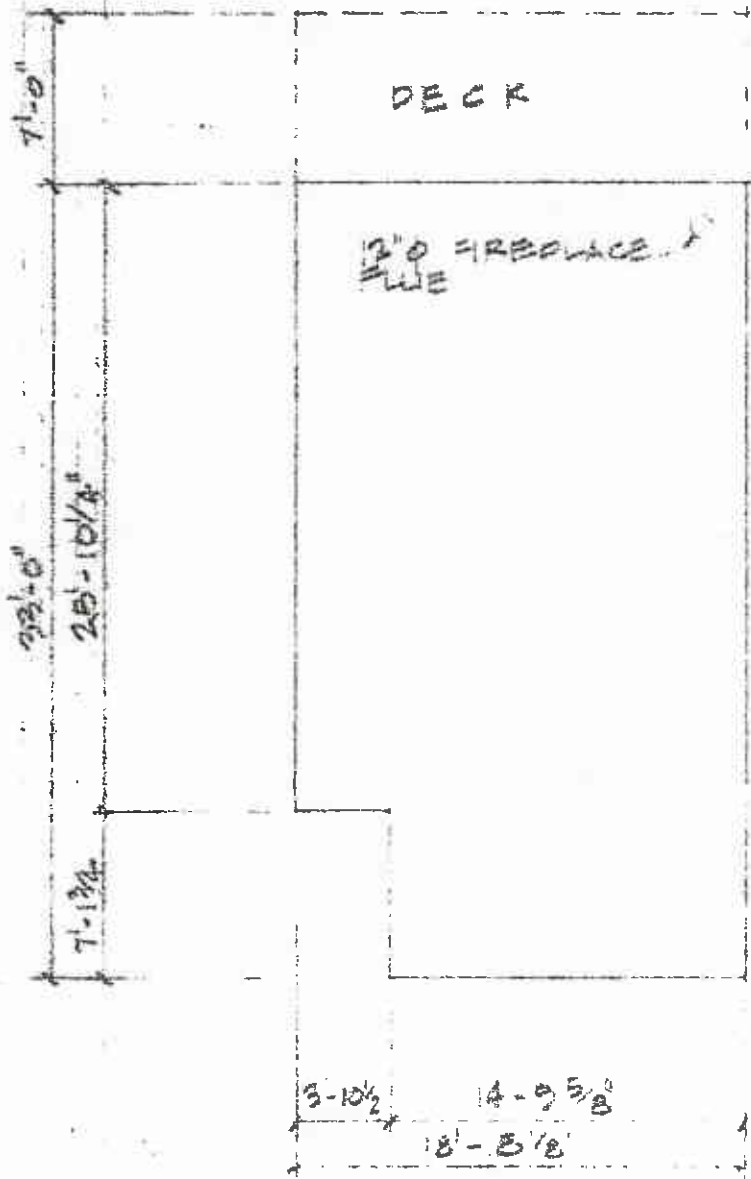
ONE BEDROOM FLOOR PLAN
